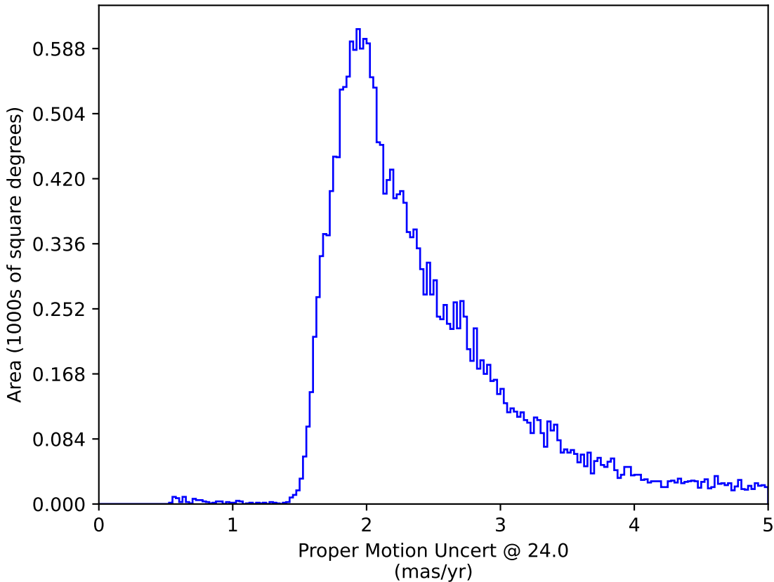
ddf_loaded_half_fl2_v3.4_10yrs : Proper Motion Uncert @ 24.0
