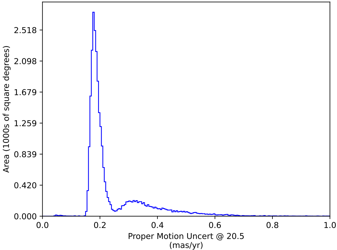
ddf_loaded_half_fl2_v3.4_10yrs : Proper Motion Uncert @ 20.5
