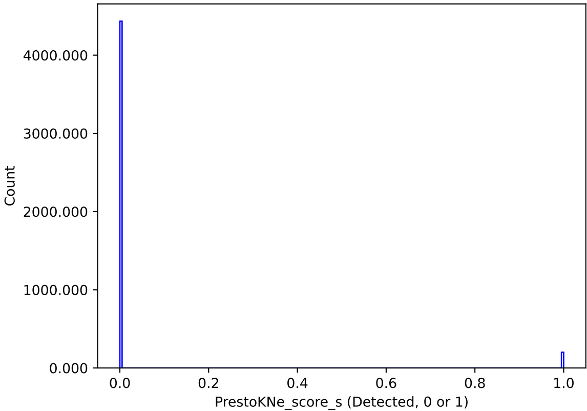
ddf_loaded_half_fl2_v3.4_10yrs : PrestoKNe_score_s
