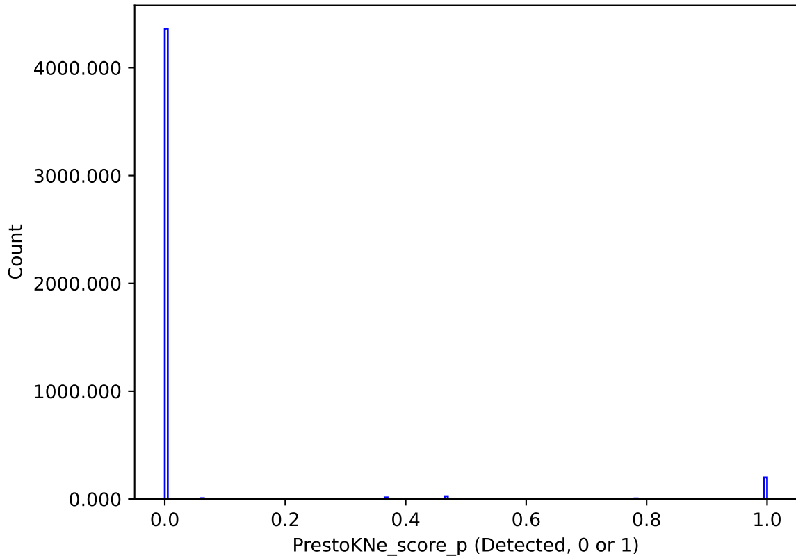
ddf_loaded_half_fl2_v3.4_10yrs : PrestoKNe_score_p
