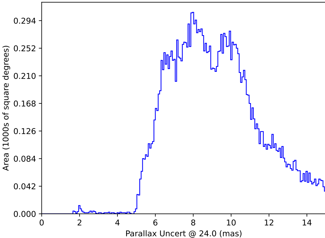
ddf_loaded_half_fl2_v3.4_10yrs : Parallax Uncert @ 24.0
