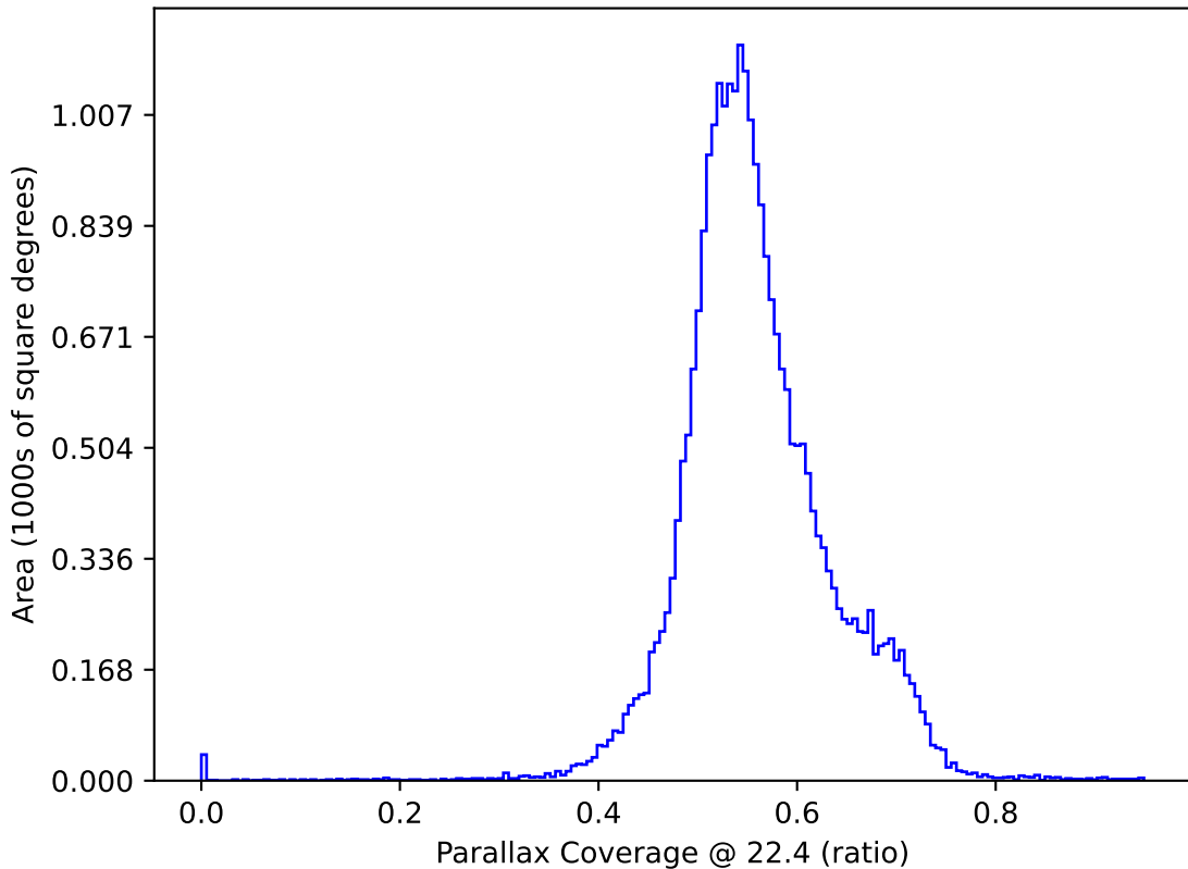
ddf_loaded_half_fl2_v3.4_10yrs : Parallax Coverage @ 22.4
