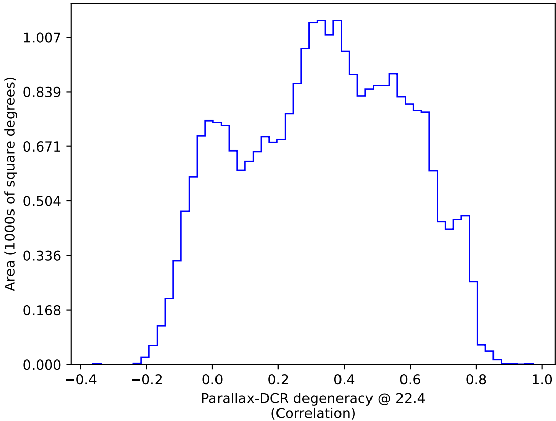
ddf_loaded_half_fl2_v3.4_10yrs : Parallax-DCR degeneracy @ 22.4
