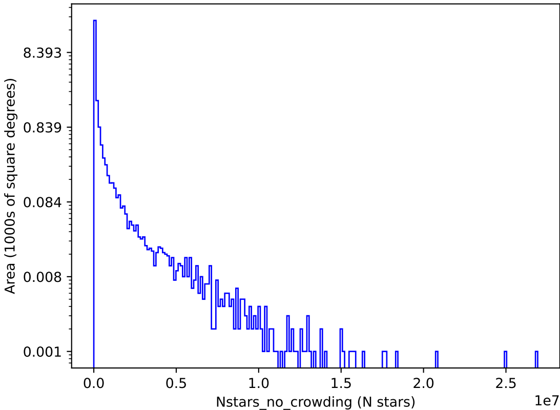
ddf_loaded_half_fl2_v3.4_10yrs z: Nstars_no_crowding
