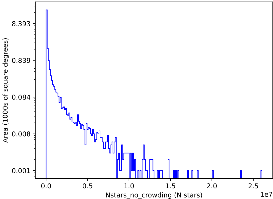
ddf_loaded_half_fl2_v3.4_10yrs y: Nstars_no_crowding
