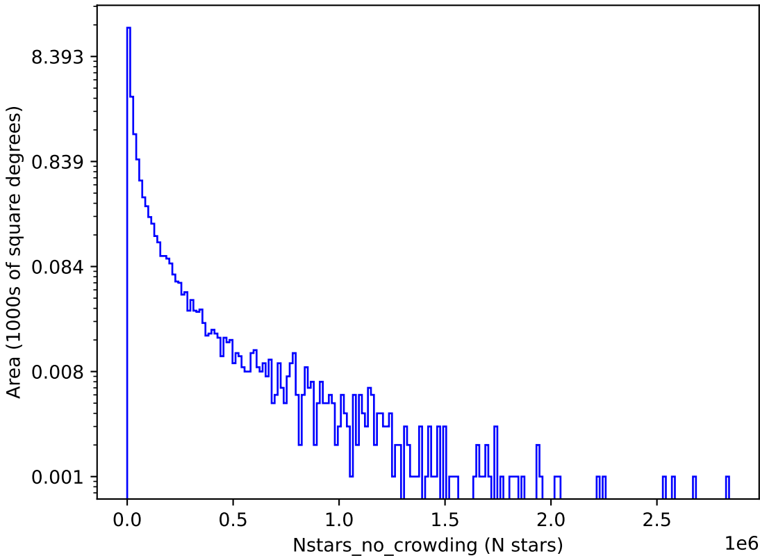
ddf_loaded_half_fl2_v3.4_10yrs u: Nstars_no_crowding
