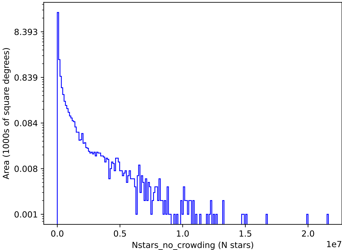
ddf_loaded_half_fl2_v3.4_10yrs r: Nstars_no_crowding
