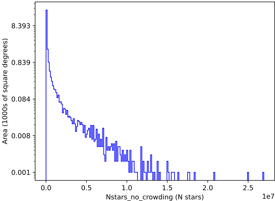
ddf_loaded_half_fl2_v3.4_10yrs i: Nstars_no_crowding
