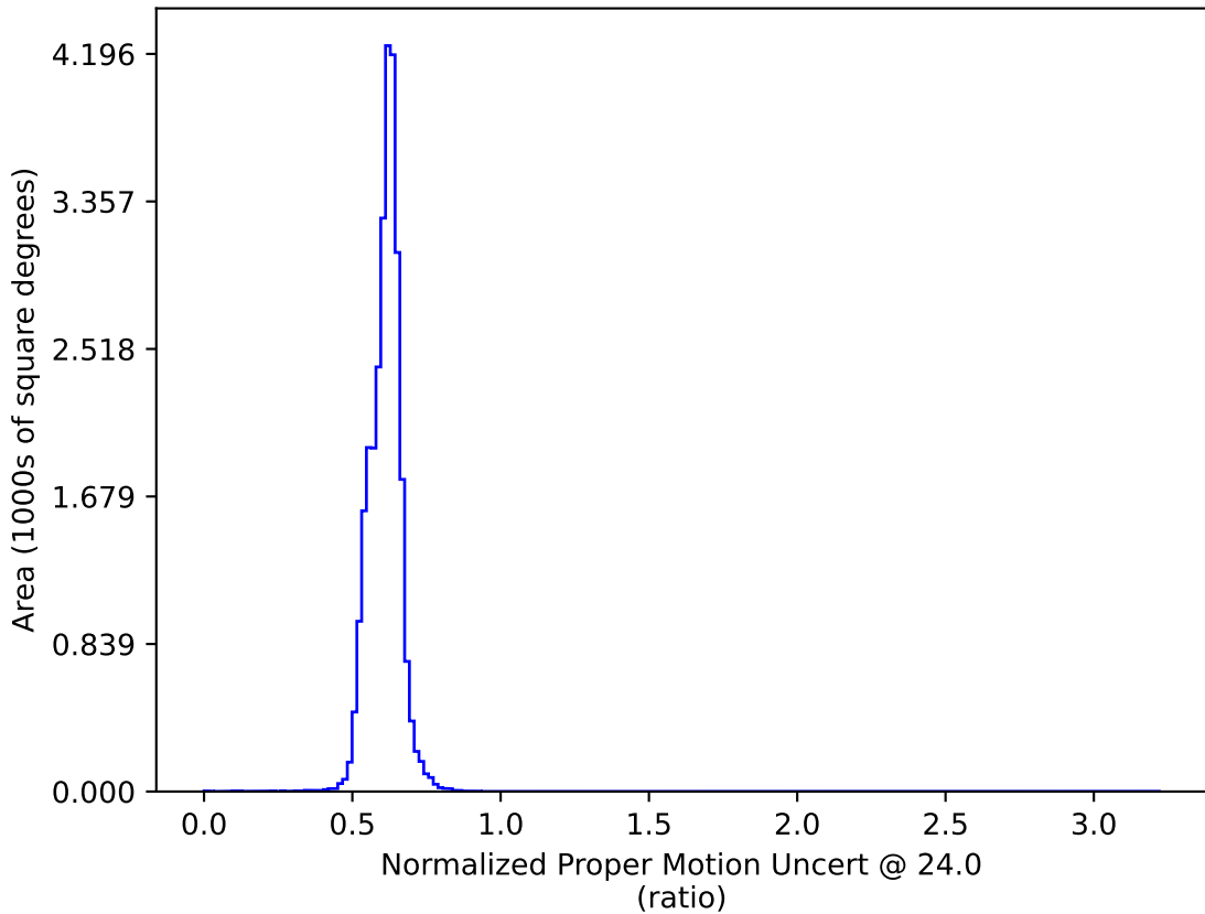
ddf_loaded_half_fl2_v3.4_10yrs : Normalized Proper Motion Uncert @ 24.0
