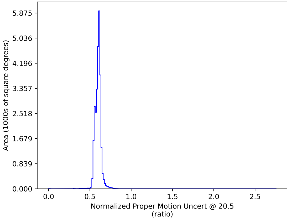
ddf_loaded_half_fl2_v3.4_10yrs : Normalized Proper Motion Uncert @ 20.5
