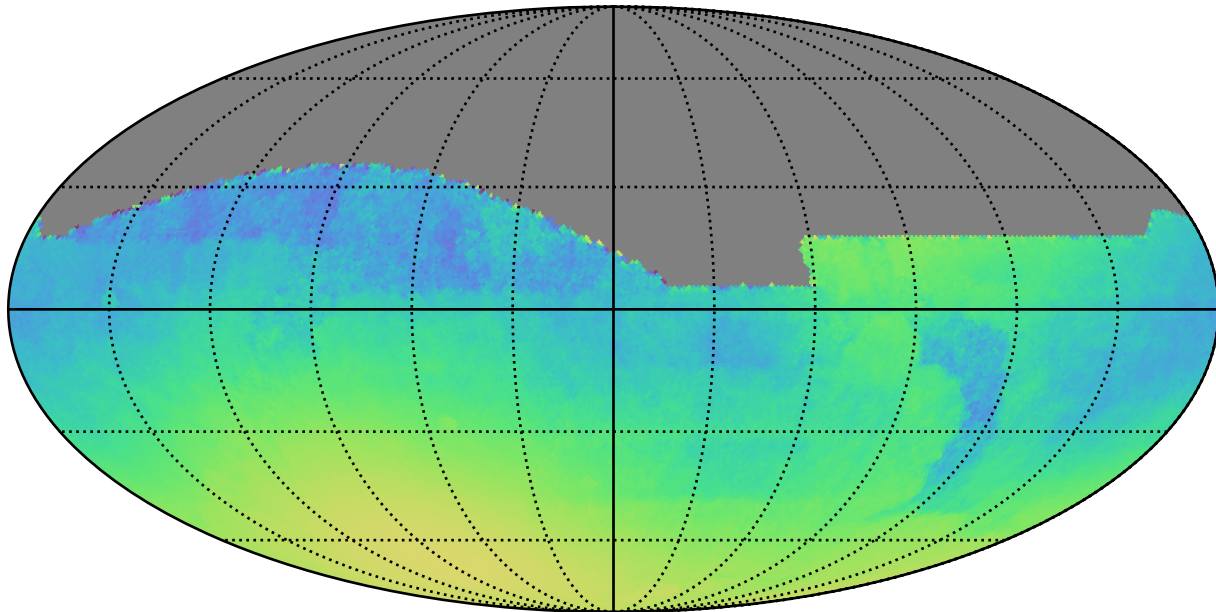
ddf_loaded_half_fl2_v3.4_10yrs : Normalized Parallax Uncert @ 24.0
