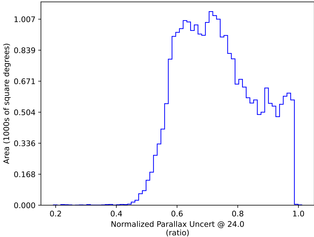
ddf_loaded_half_fl2_v3.4_10yrs : Normalized Parallax Uncert @ 24.0
