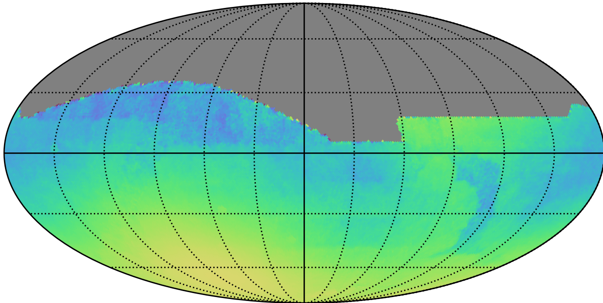
ddf_loaded_half_fl2_v3.4_10yrs : Normalized Parallax Uncert @ 22.4
