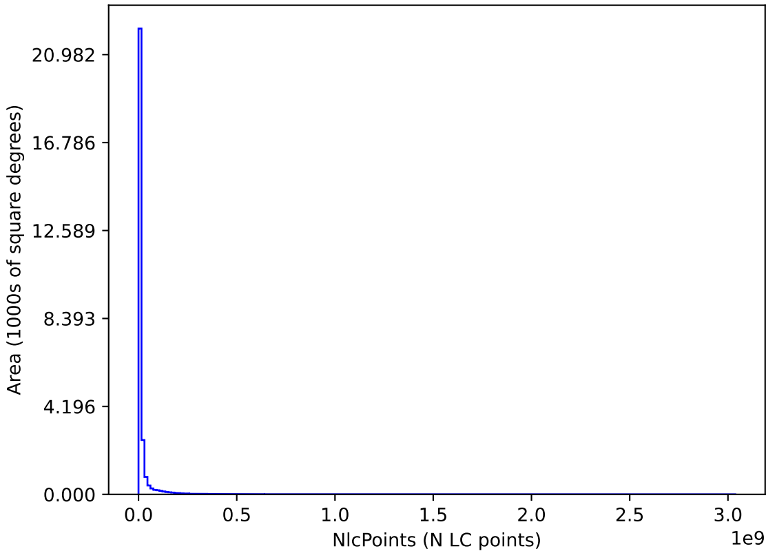
ddf_loaded_half_fl2_v3.4_10yrs : NlcPoints
