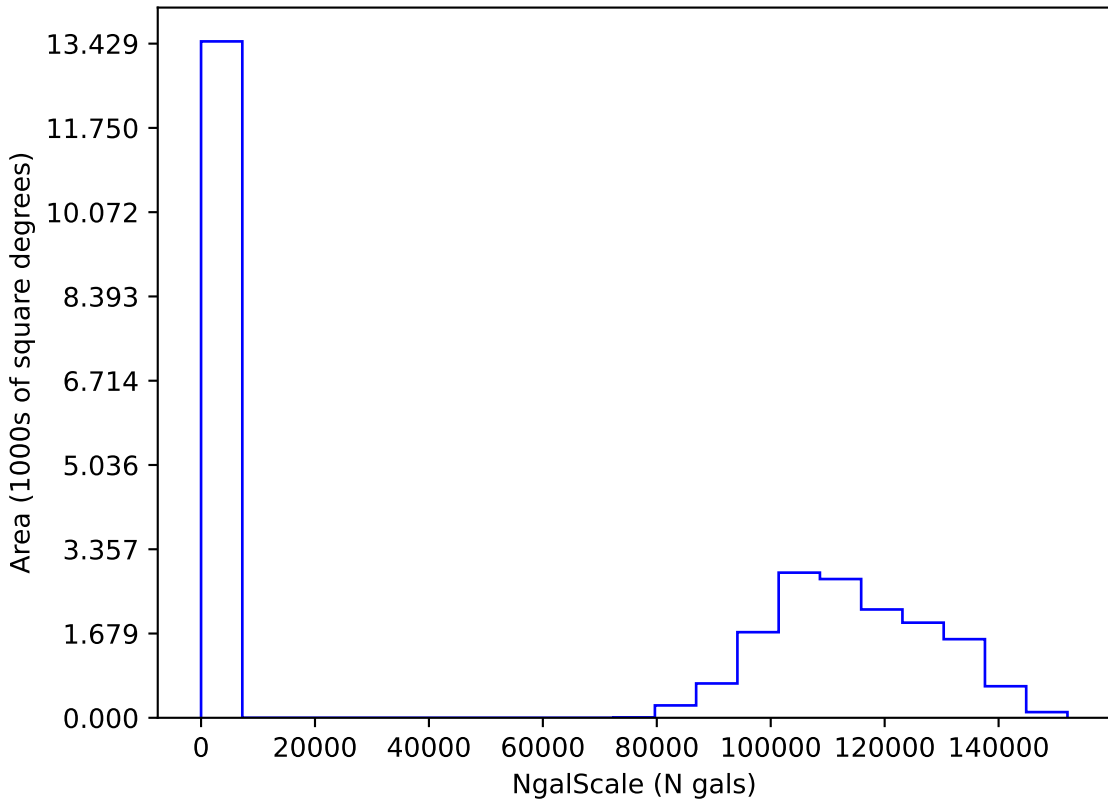
ddf_loaded_half_fl2_v3.4_10yrs i: NgalScale
