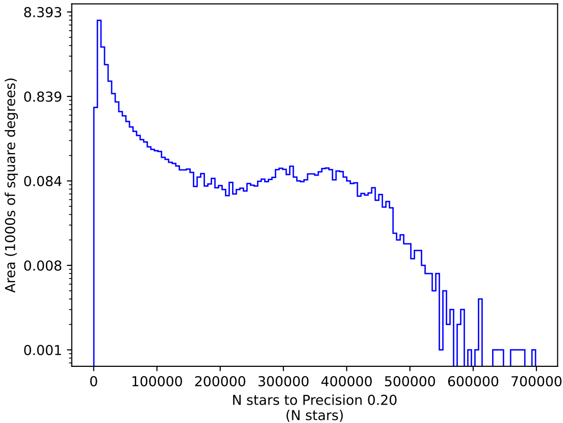
ddf_loaded_half_fl2_v3.4_10yrs y: N stars to Precision 0.20
