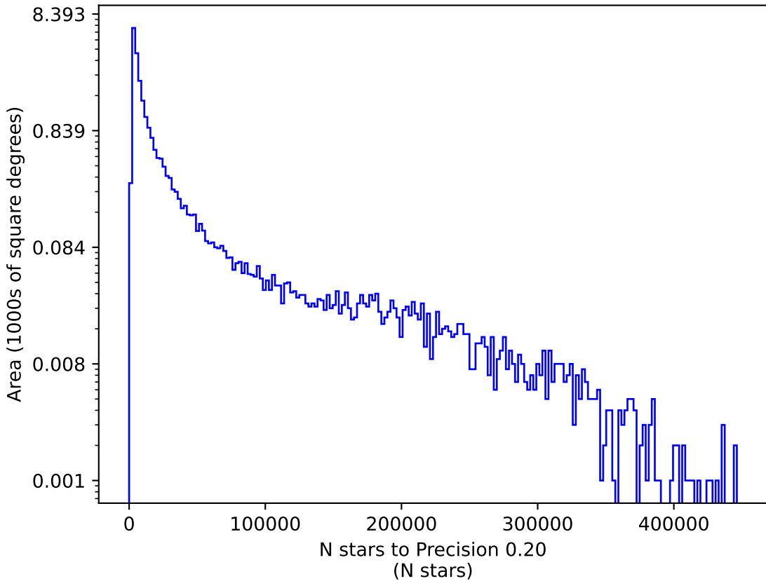
ddf_loaded_half_fl2_v3.4_10yrs u: N stars to Precision 0.20
