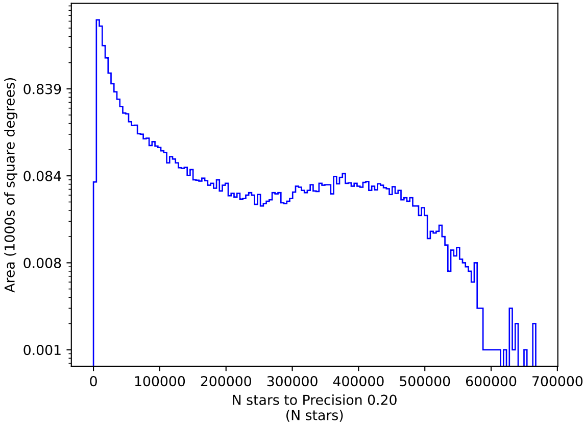
ddf_loaded_half_fl2_v3.4_10yrs r: N stars to Precision 0.20
