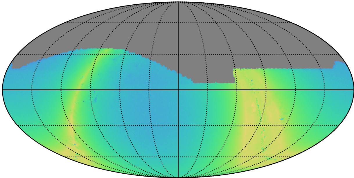
ddf_loaded_half_fl2_v3.4_10yrs i: N stars to Precision 0.20
