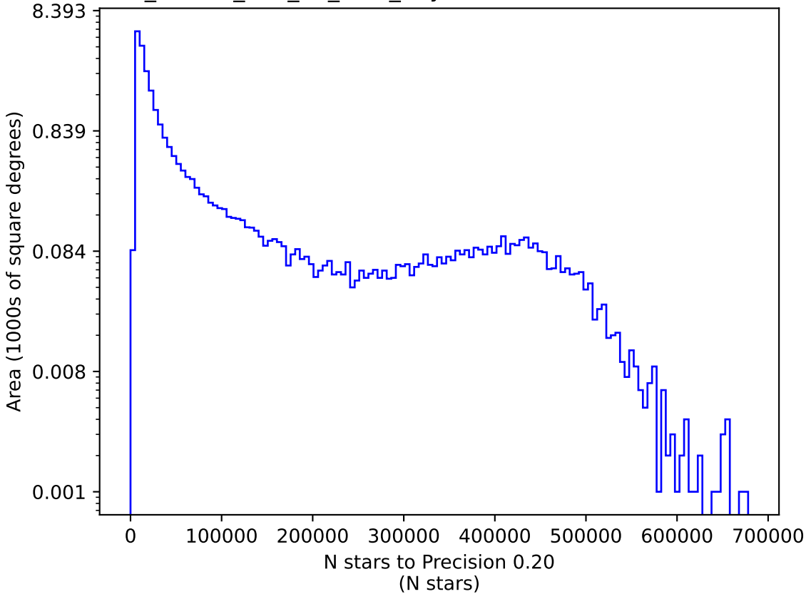
ddf_loaded_half_fl2_v3.4_10yrs i: N stars to Precision 0.20
