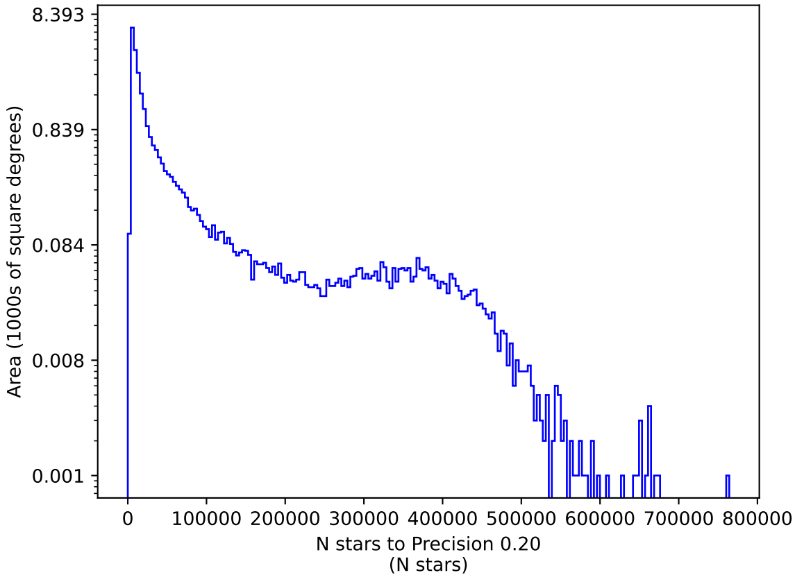
ddf_loaded_half_fl2_v3.4_10yrs g: N stars to Precision 0.20
