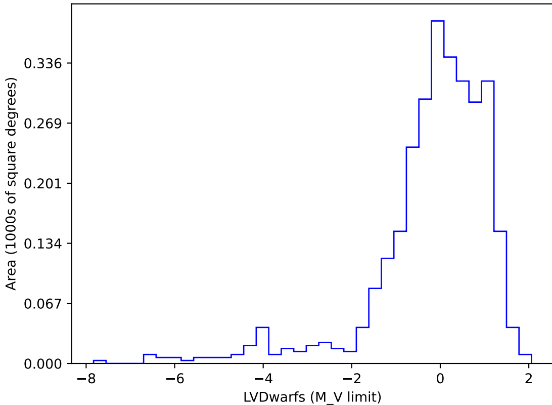
ddf_loaded_half_fl2_v3.4_10yrs gi SCP: LVDwarfs
