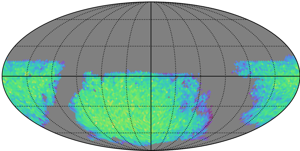
ddf_loaded_half_fl2_v3.4_10yrs gi: LVDwarfs
