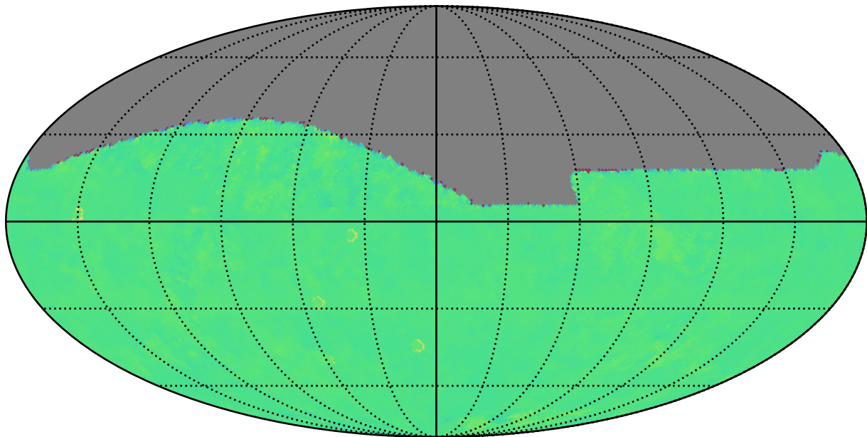
ddf_loaded_half_fl2_v3.4_10yrs z: Kuiper rotTelPos
