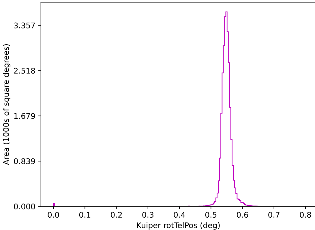
ddf_loaded_half_f12_v3.4_10yrs z: Kuiper rotTelPos
