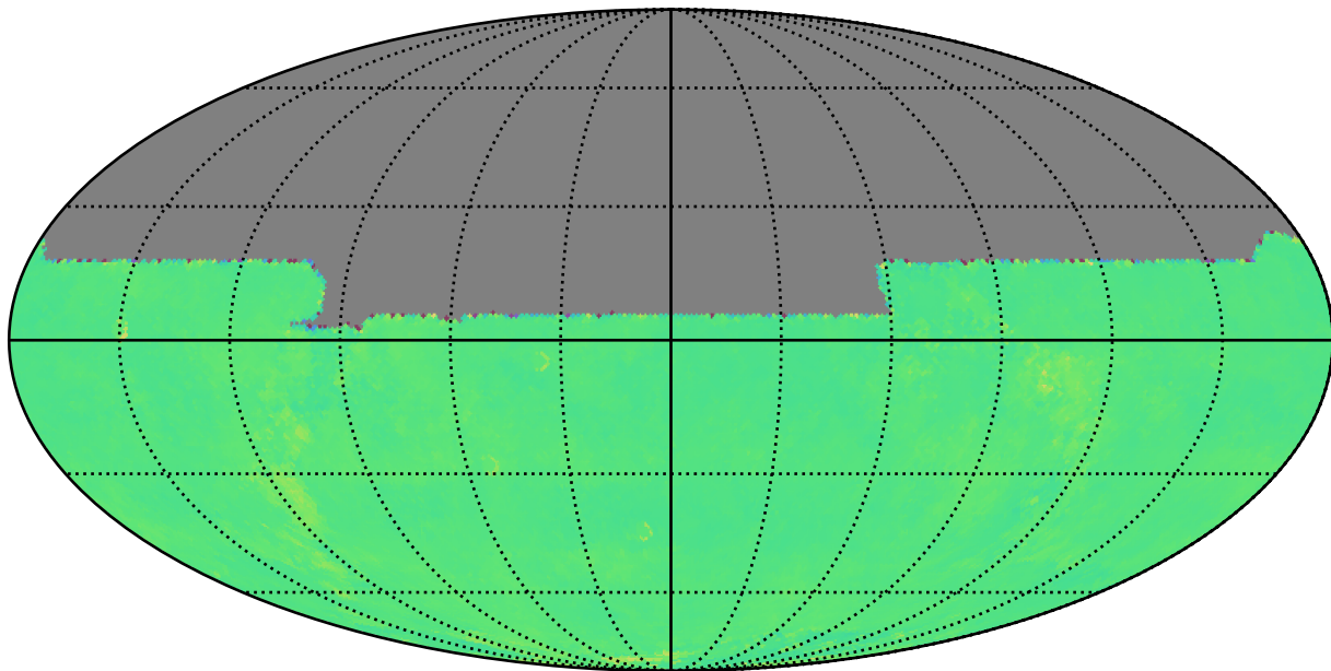
ddf_loaded_half_fl2_v3.4_10yrs y: Kuiper rotTelPos
