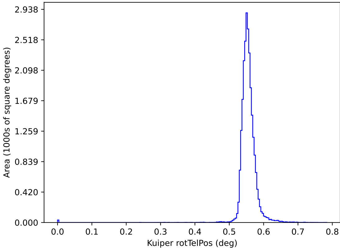
ddf_loaded_half_f12_v3.4_10yrs y: Kuiper rotTelPos
