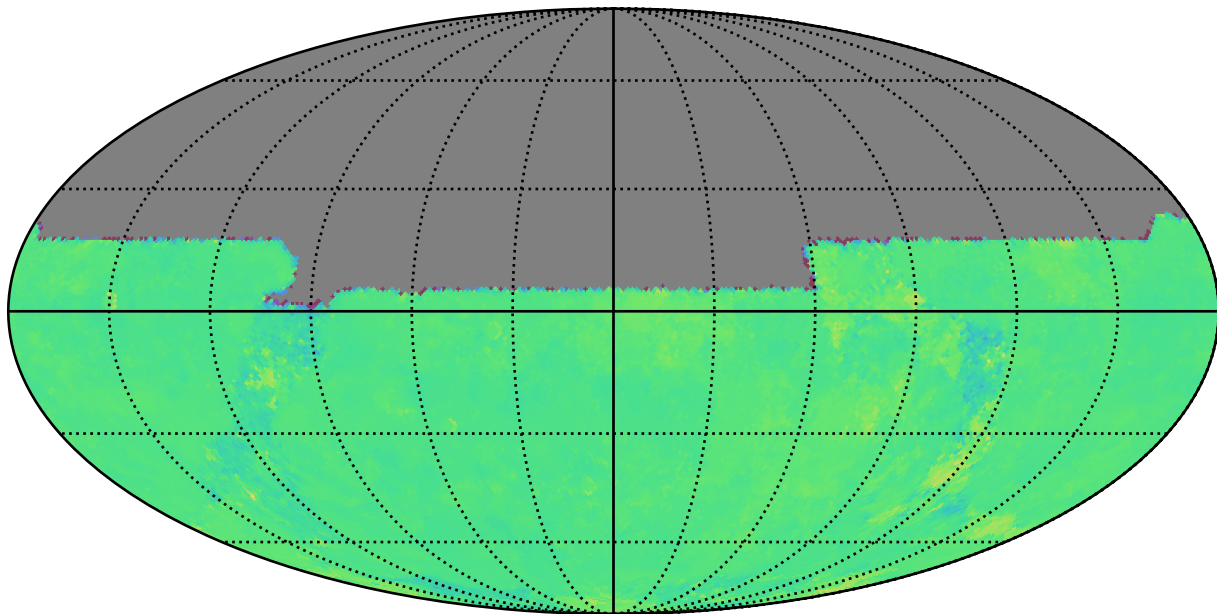
ddf_loaded_half_fl2_v3.4_10yrs u: Kuiper rotTelPos
