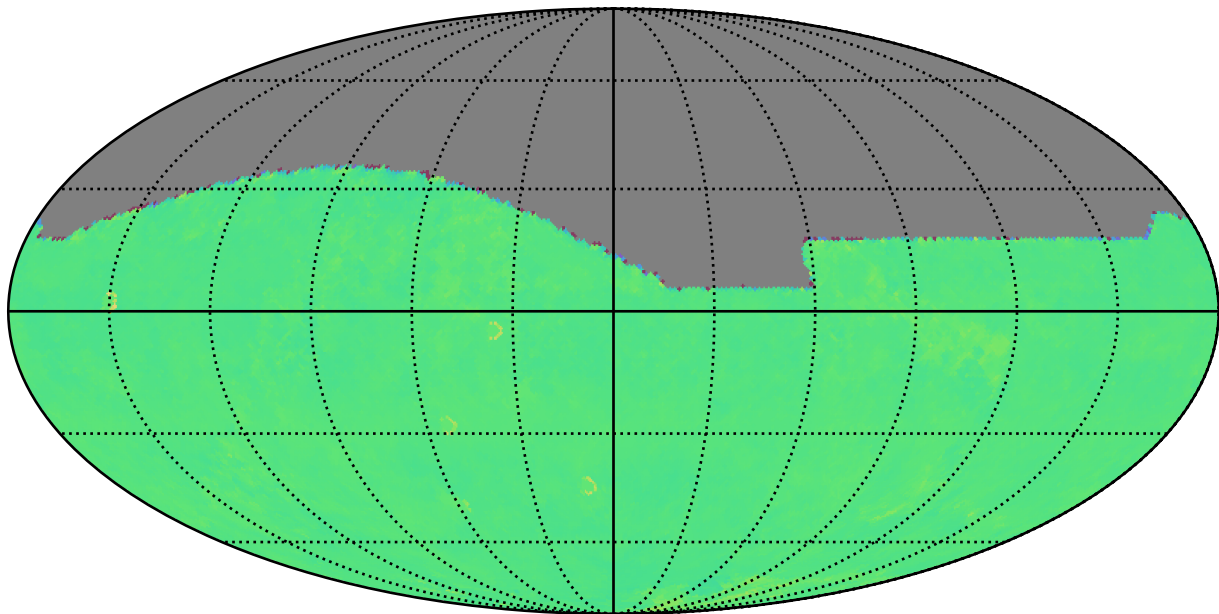
ddf_loaded_half_fl2_v3.4_10yrs i: Kuiper rotTelPos
