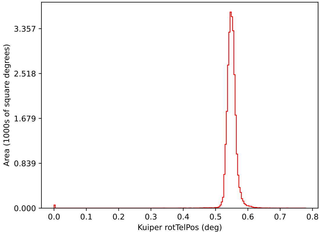
ddf_loaded_half_fl2_v3.4_10yrs i: Kuiper rotTelPos
