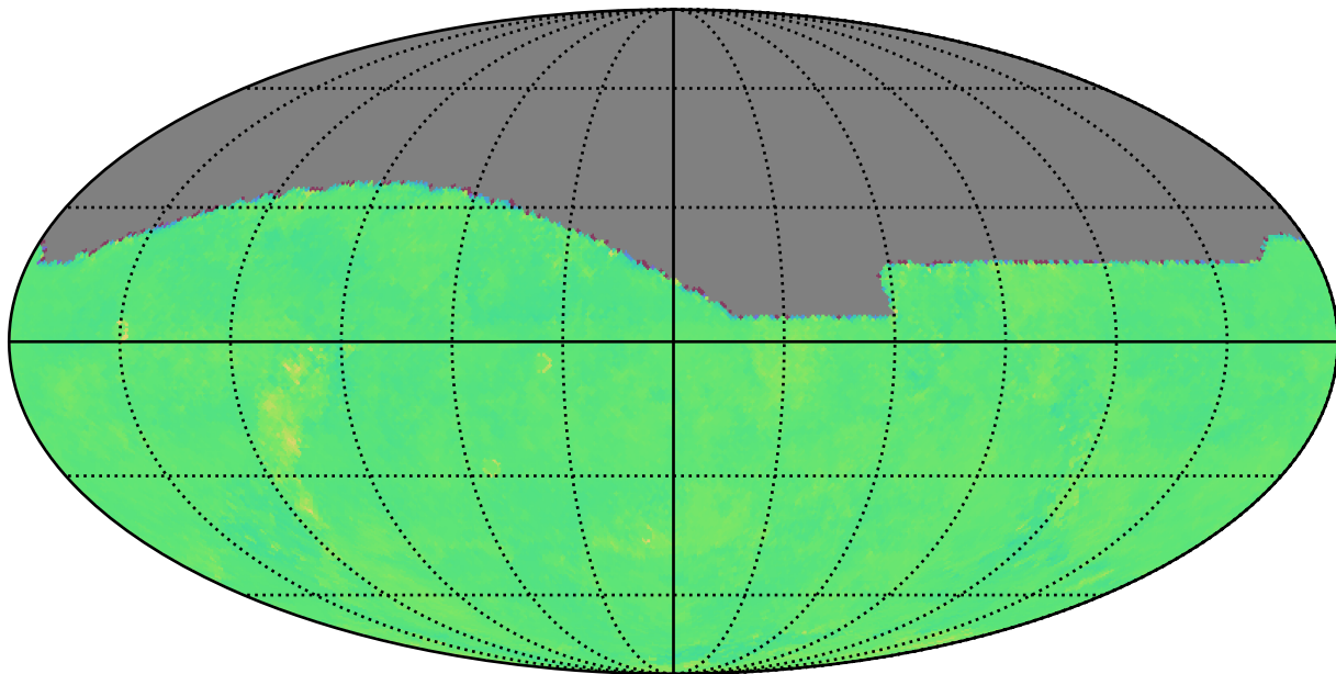
ddf_loaded_half_fl2_v3.4_10yrs g: Kuiper rotTelPos
