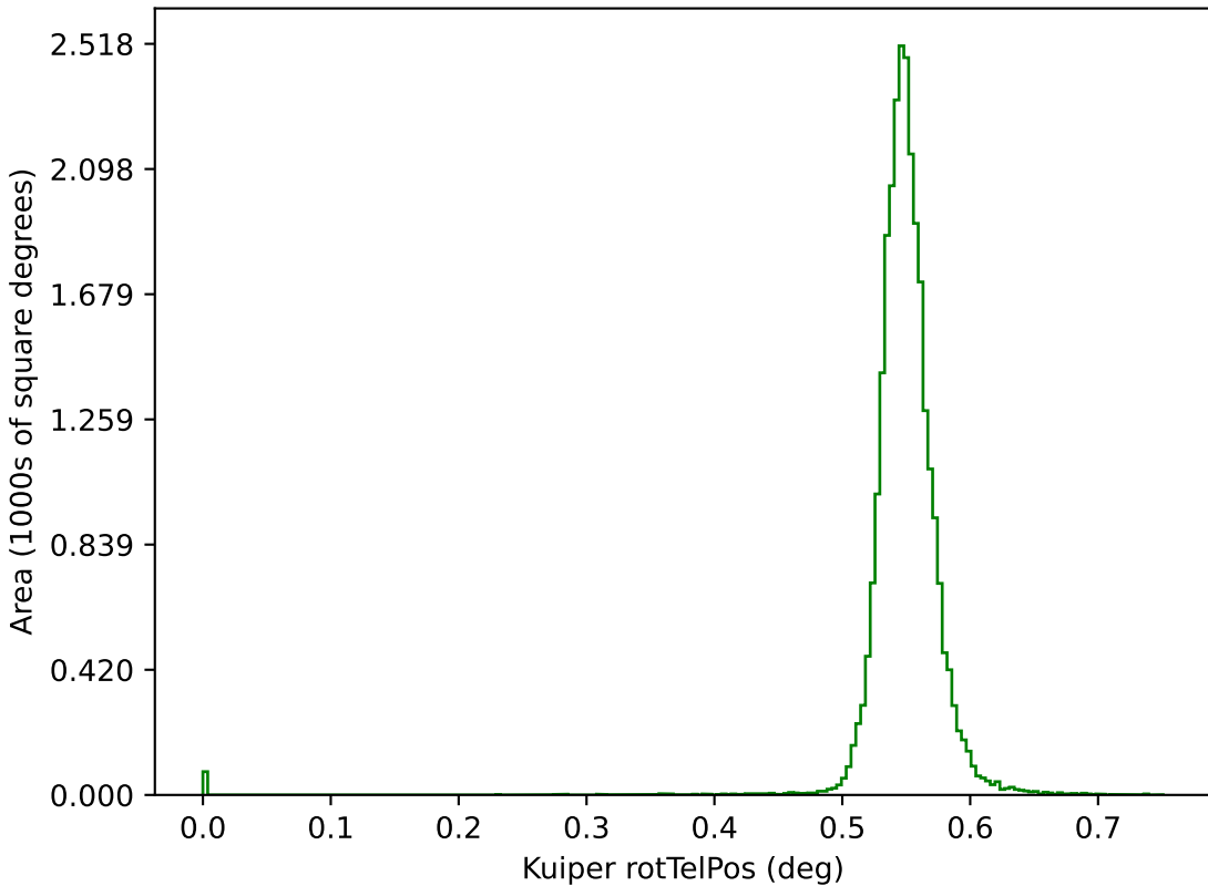
ddf_loaded_half_fl2_v3.4_10yrs g: Kuiper rotTelPos
