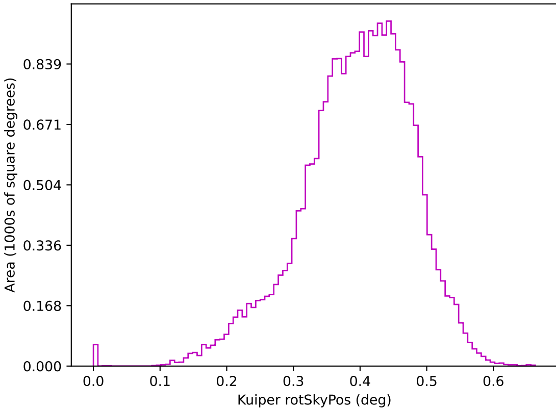
ddf_loaded_half_fl2_v3.4_10yrs z: Kuiper rotSkyPos
