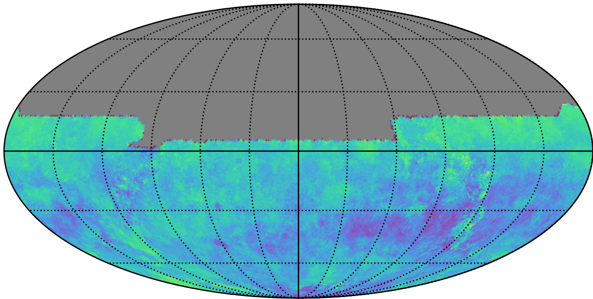
ddf_loaded_half_fl2_v3.4_10yrs u: Kuiper rotSkyPos
