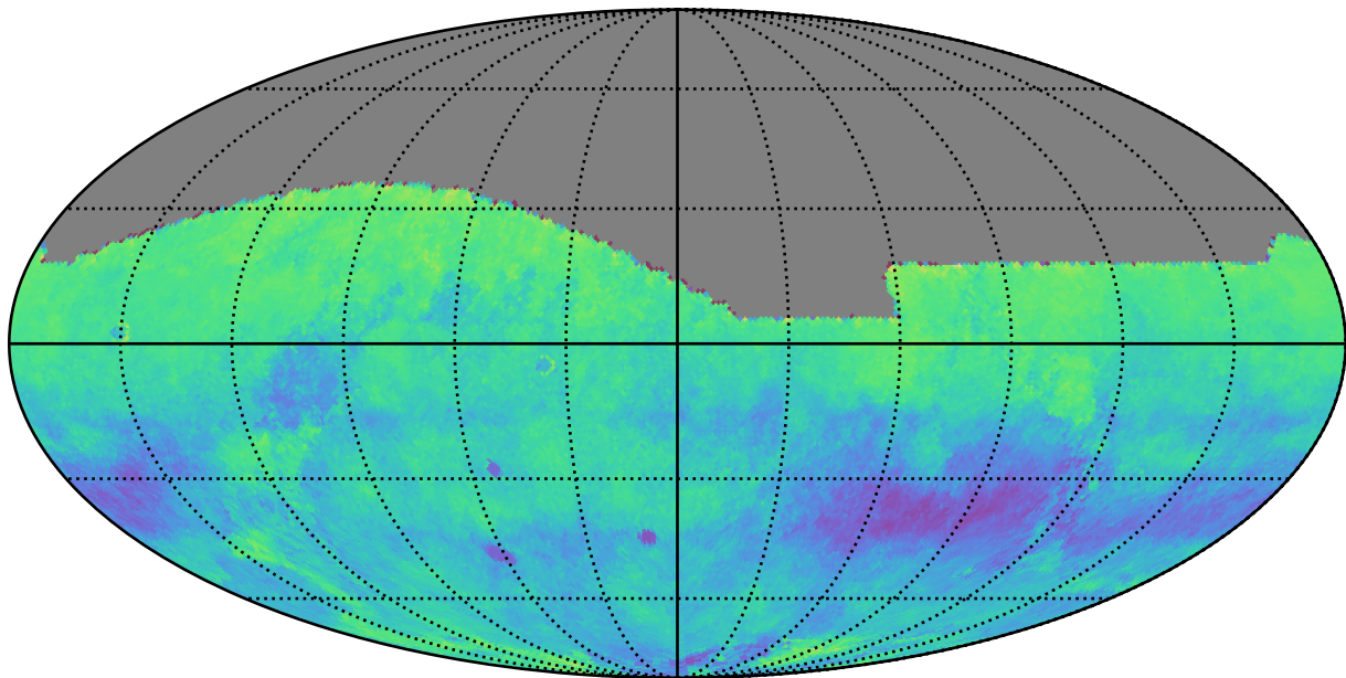
ddf_loaded_half_fl2_v3.4_10yrs r: Kuiper rotSkyPos
