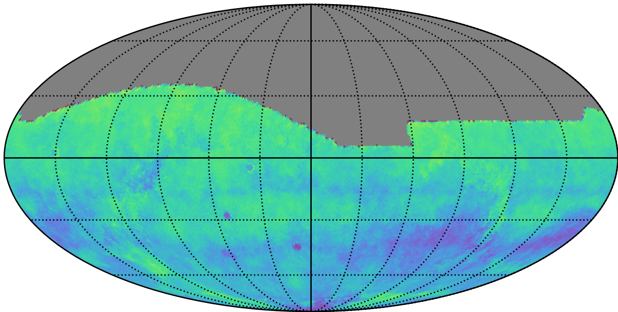
ddf_loaded_half_fl2_v3.4_10yrs i: Kuiper rotSkyPos
