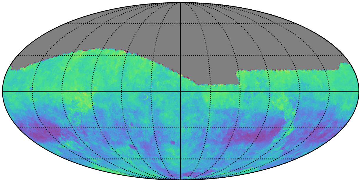
ddf_loaded_half_fl2_v3.4_10yrs g: Kuiper rotSkyPos
