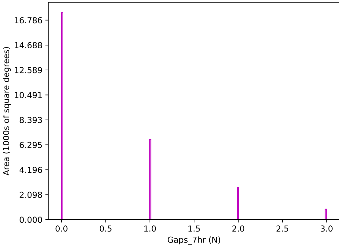
ddf_loaded_half_fl2_v3.4_10yrs z band: Gaps_7hr
