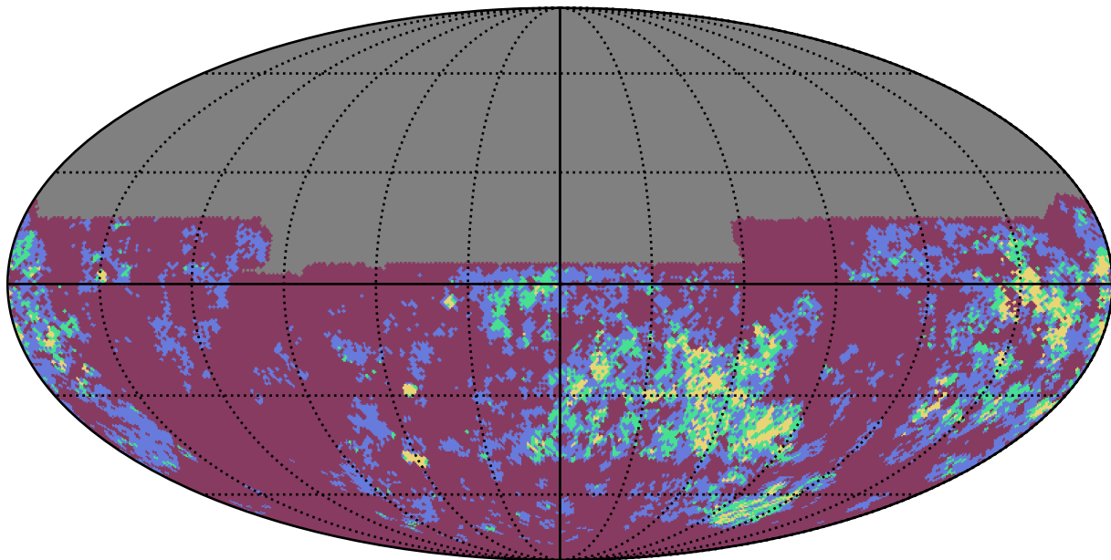
ddf_loaded_half_fl2_v3.4_10yrs y band: Gaps_7hr
