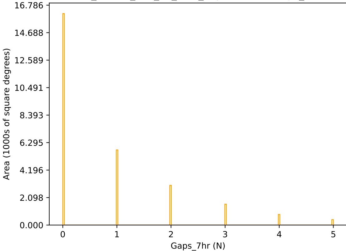
ddf_loaded_half_fl2_v3.4_10yrs r band: Gaps_7hr
