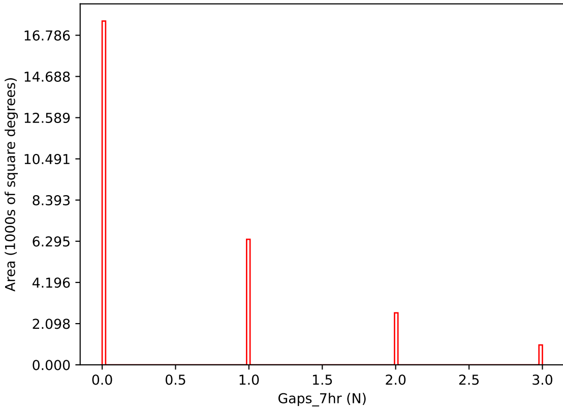
ddf_loaded_half_fl2_v3.4_10yrs i band: Gaps_7hr
