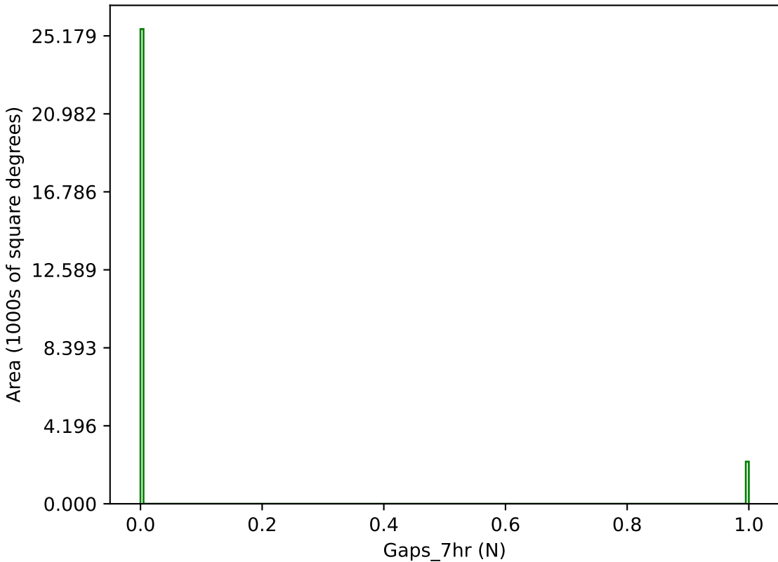
ddf_loaded_half_fl2_v3.4_10yrs g band: Gaps_7hr
