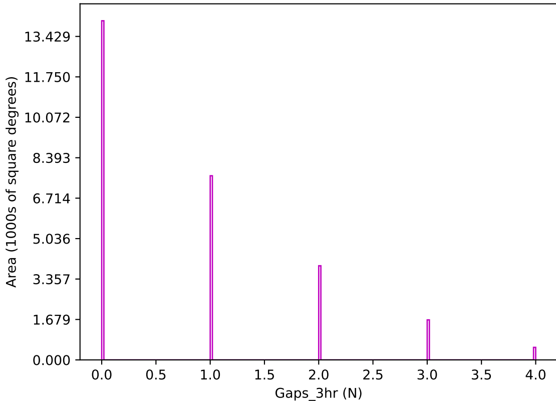
ddf_loaded_half_fl2_v3.4_10yrs z band: Gaps_3hr
