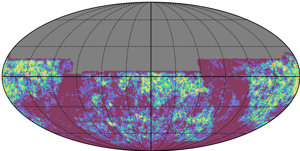
ddf_loaded_half_fl2_v3.4_10yrs y band: Gaps_3hr
