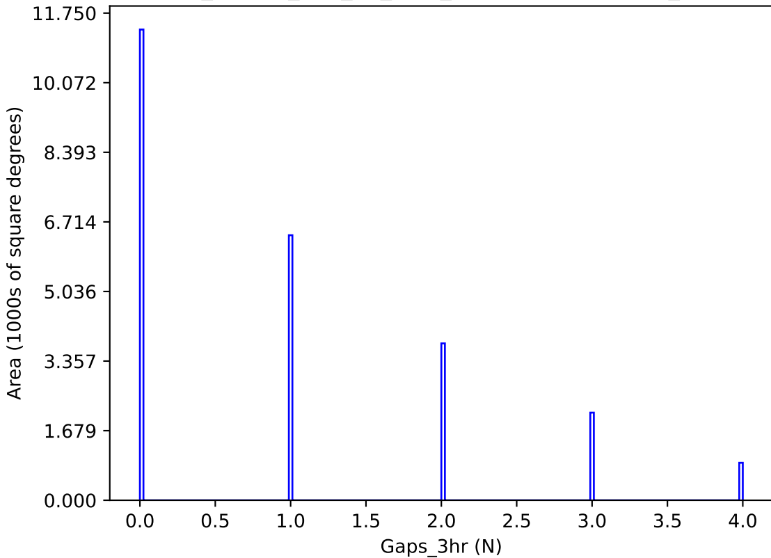
ddf_loaded_half_fl2_v3.4_10yrs y band: Gaps_3hr
