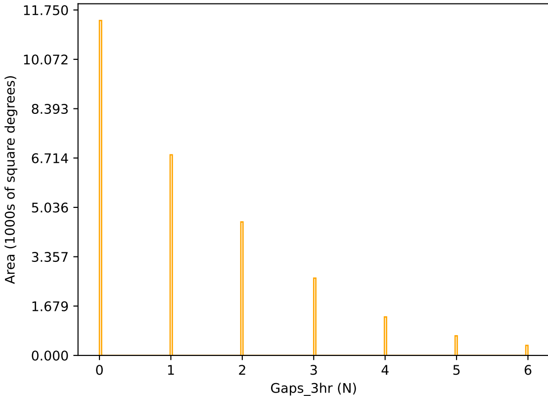
ddf_loaded_half_fl2_v3.4_10yrs r band: Gaps_3hr
